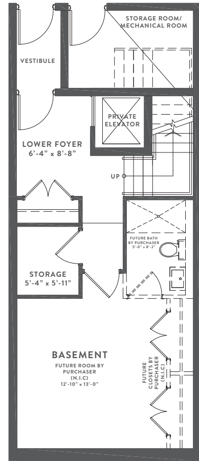
LOWER LEVEL 220 sq. ft.
